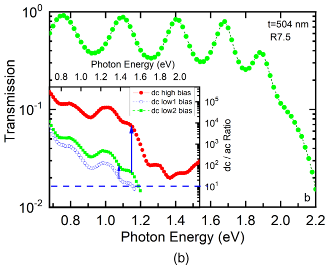
FIG. 2. (a) Relative DBP yield spectra of undoped a-Si:H in the annealed state measured with three different dc bias light intensities. In the inset, the phase of DBP signals is shown for corresponding dc bias light measurements. (b) Optical transmission spectrum in absolute scale simultaneously measured from the back of the sample. In the inset, dc/ac ratios of photocurrents are presented for each DBP measurement.
