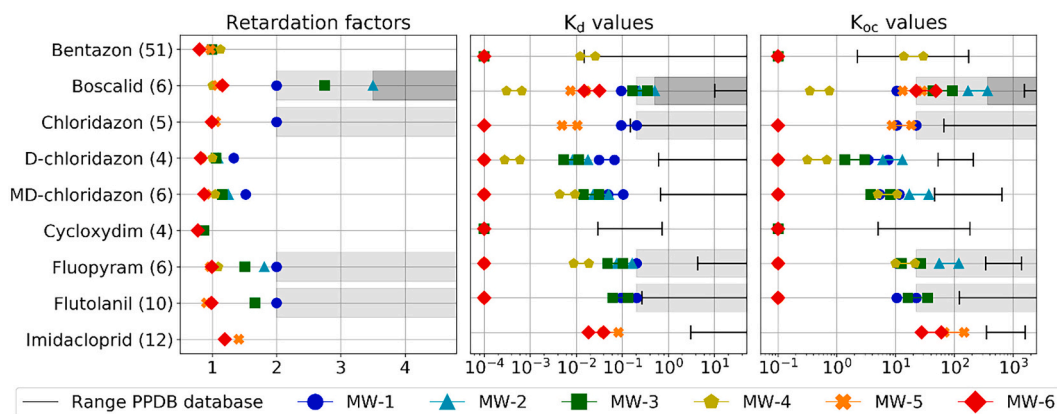
Fig. 3. Calculated pesticide retardation factors (R), partition coefficients ( K_d ), and organic carbon-water partition coefficients ( K_{oc} ). Retardation factors are not shown for model fits with r^2 < 0.7 . The different colors and symbols present the data from the different well screen depths. The light and dark grey background indicates R > 2.0 and R > 3.5 respectively, and the K_d and K_{oc} that are determined based on this R. K_d = 0 were set to 10^{-4} and K_{oc} = 0 were set to 10^{-1} . The minimum K_d and K_{oc} is calculated based on \epsilon = 0.2 , and the maximum based on \epsilon = 0.35 , based on Table 3.1 from Appelo and Postma (2004). The ranges in black present the PPDB database ranges. The number in parenthesis behind the pesticide names show the number of studied soils which are reported in the PPDB database.
