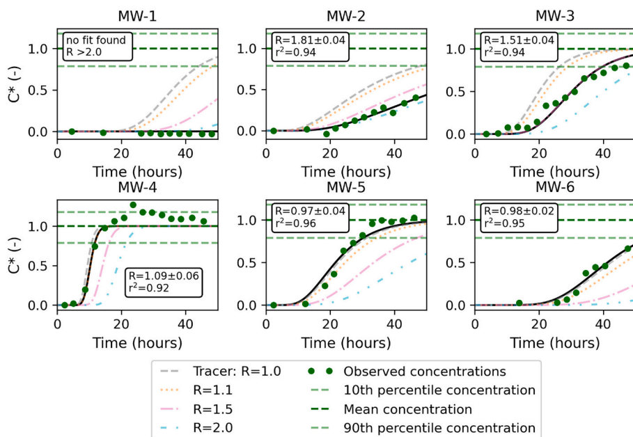
Fig. 2. Retardation factor (R) of fluopyram at different aquifer depths. The green dots show the normalized observed concentrations. The black line shows the best fit to these concentrations, from which R was obtained. The mean injected concentration is shown with a dashed dark green line, its 10% and 90% percentiles with light green dashed lines. The dashed, grey, orange, pink, and cyan lines display breakthrough with indicated R values. (For interpretation of the references to colour in this figure legend, the reader is referred to the web version of this article.)
