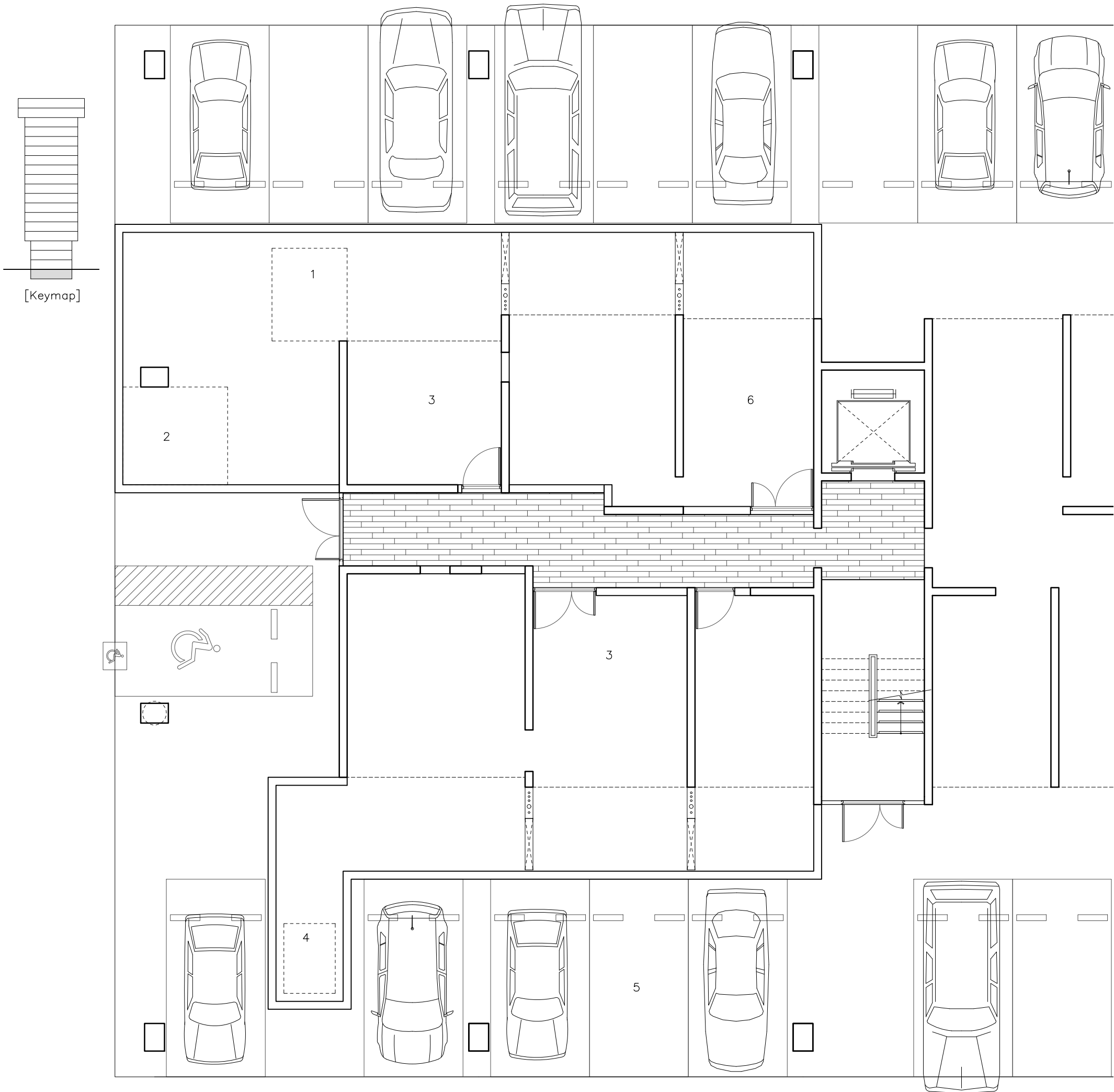
[Basement Floor]
