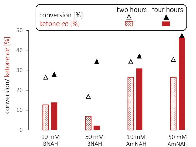
Fig. 2 Screening of the NCB-driven chemo-enzymatic enantioselective BV oxidation of rac - 1 by 2,5-DCKMO. Conversion (%), (▲) and ketone 1 ee (%), (■, red bars) after, respectively, two and four hours as the average of duplicates. Experimental conditions: 5 mM rac - 1 , 0.55 mg mL -1 purified and lyophilized oxygenase, 0.5 mg mL -1 catalase, and 100 μM FMN in 1 mL of Tris-HCl buffer (50 mM, pH 7.5 at 22 °C).
