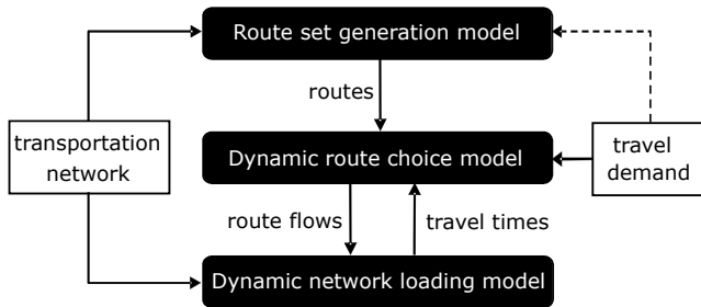
Fig. 1. Structure of a dynamic traffic assignment model
