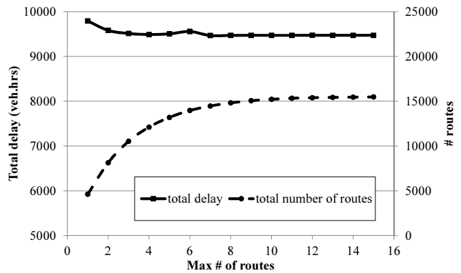
Fig. 8. Total Delay and Number of Routes for Case 2
