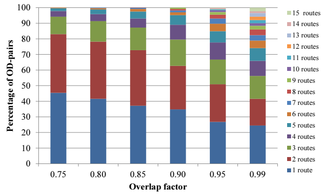
Fig. 5. Frequency of Routes for Case 1
