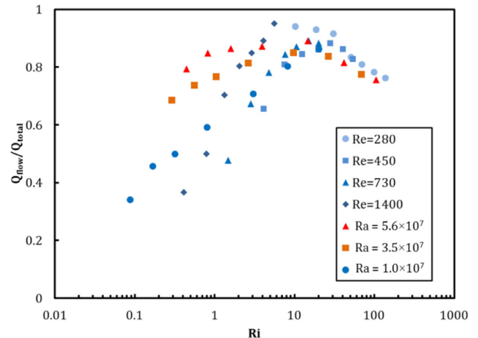
Fig. 15. The ratio Q_{\text{flow}}/Q_{\text{total}} as a function of Richardson number for all experiments (configuration A).
