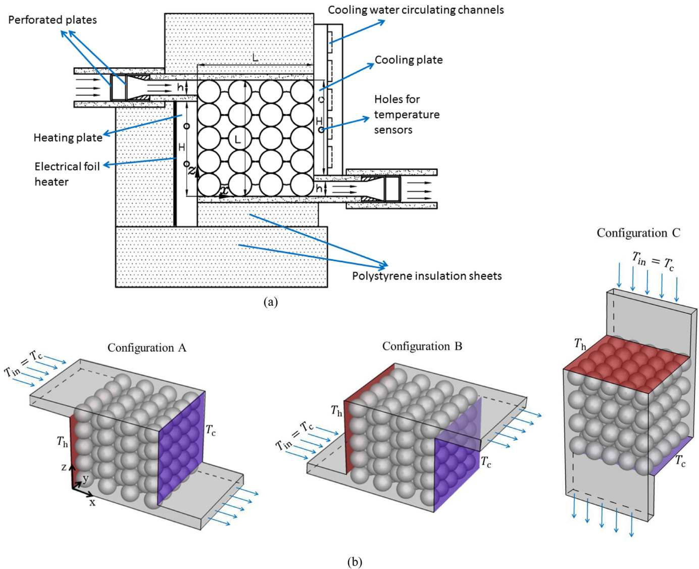
Fig. 1. The mixed convection cavity filled with d/L = 0.20 spheres in BCT packing: (a) Drawing and components of the cavity (configuration A), (b) Schematic view of the two studied mixed convection configurations A and B, and the pure forced convection configuration C. In all experiments the same cavity was used positioned in three different ways (Configuration A, B, and C). Results will be presented in the Cartesian coordinate system shown in Fig. 1b.
