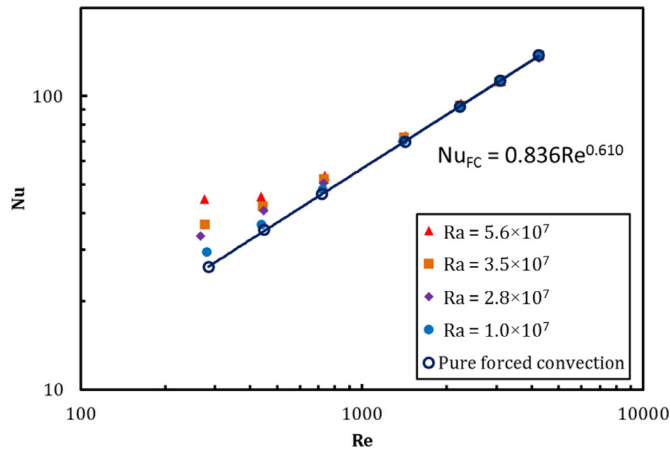
Fig. 5. Nu-Re data for the porous medium filled cavity for different Rayleigh numbers (configuration A). The solid line shows the power-law fit to the pure forced convection data, Eq. (6), for the same cavity.
