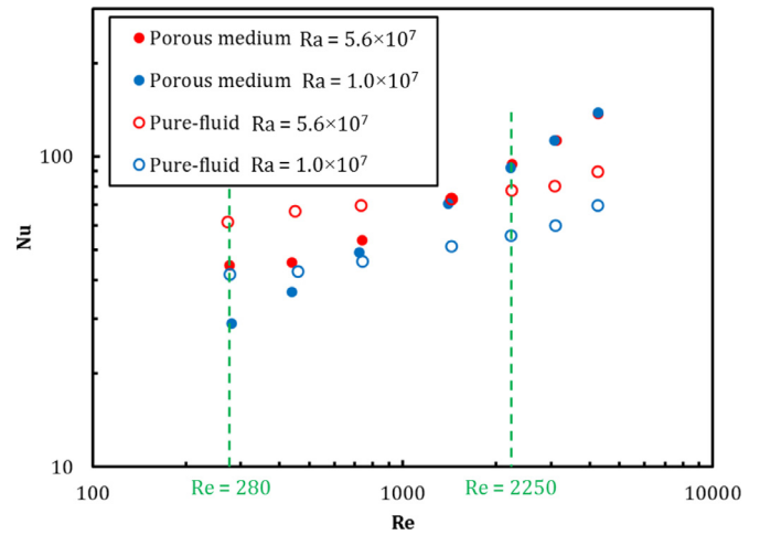
Fig. 2. Nu-Re data for the porous medium filled cavity compared to the pure-fluid cavity at two different Rayleigh numbers in configuration A.
