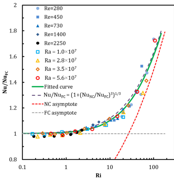
Fig. 10. Nusselt number, Nu , normalized with the pure forced convection Nusselt number, Nu_{FC} , as a function of Richardson number, Ri (configuration A). The (green) solid line shows the curve that was fitted to the data according to Eq. (7). The dashed line pertains to the correlation in Eq. (9).
