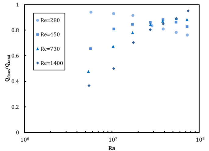
Fig. 14. The ratio Q_{\text{flow}}/Q_{\text{total}} as a function of Rayleigh number for different Reynolds numbers in configuration A.
