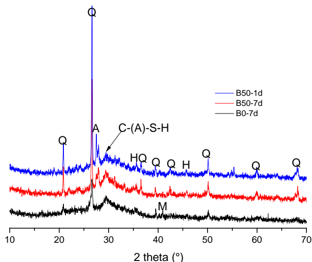
Figure 5: XRD patterns of hardened paste (Q: quartz, M: mullite, H: hematite A: albite)
