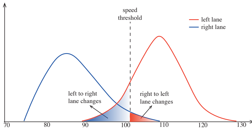
Figure 1: Desired speed distribution functions per lane for a hypothetical 2-lane section, showing the concept of threshold speed.
