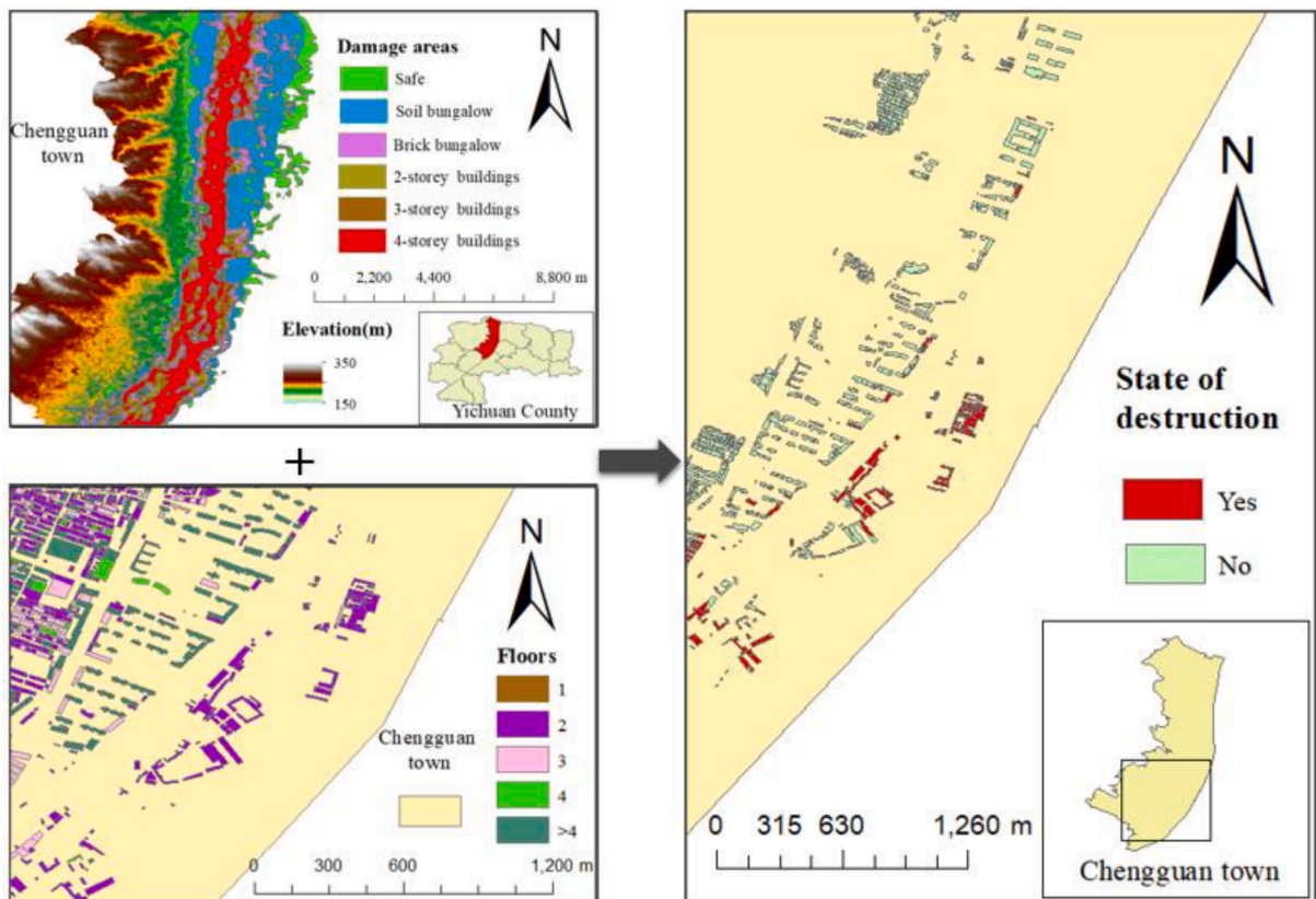
Fig. 5. Damage of buildings in Chengguan Town.
