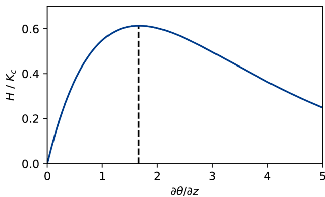
Fig. 13. The heat flux H (scaled by K_c ), shown against the temperature gradient. With an increasing gradient, the heat flux will increase up to \frac{\partial\theta}{\partial z} \approx \sim 1.67 \text{ K m}^{-1} , after which the heat flux decreases with increasing gradient. The maximum sustainable heat flux is illustrated by the dashed line, which is at \frac{\partial\theta}{\partial z} = \alpha^{-1} \text{ K m}^{-1}
