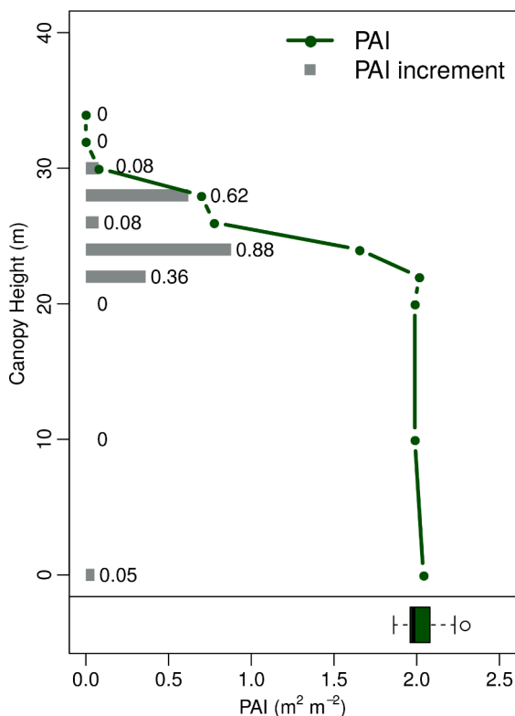
Fig. C.1. Profile of the plant area index (PAI) at the Speulderbos site (Schilperoort et al., 2020).
