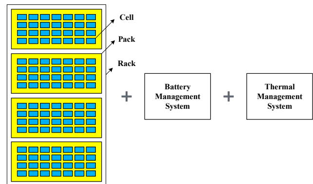
Fig. 2. The overview of the typical components in a BESS.
