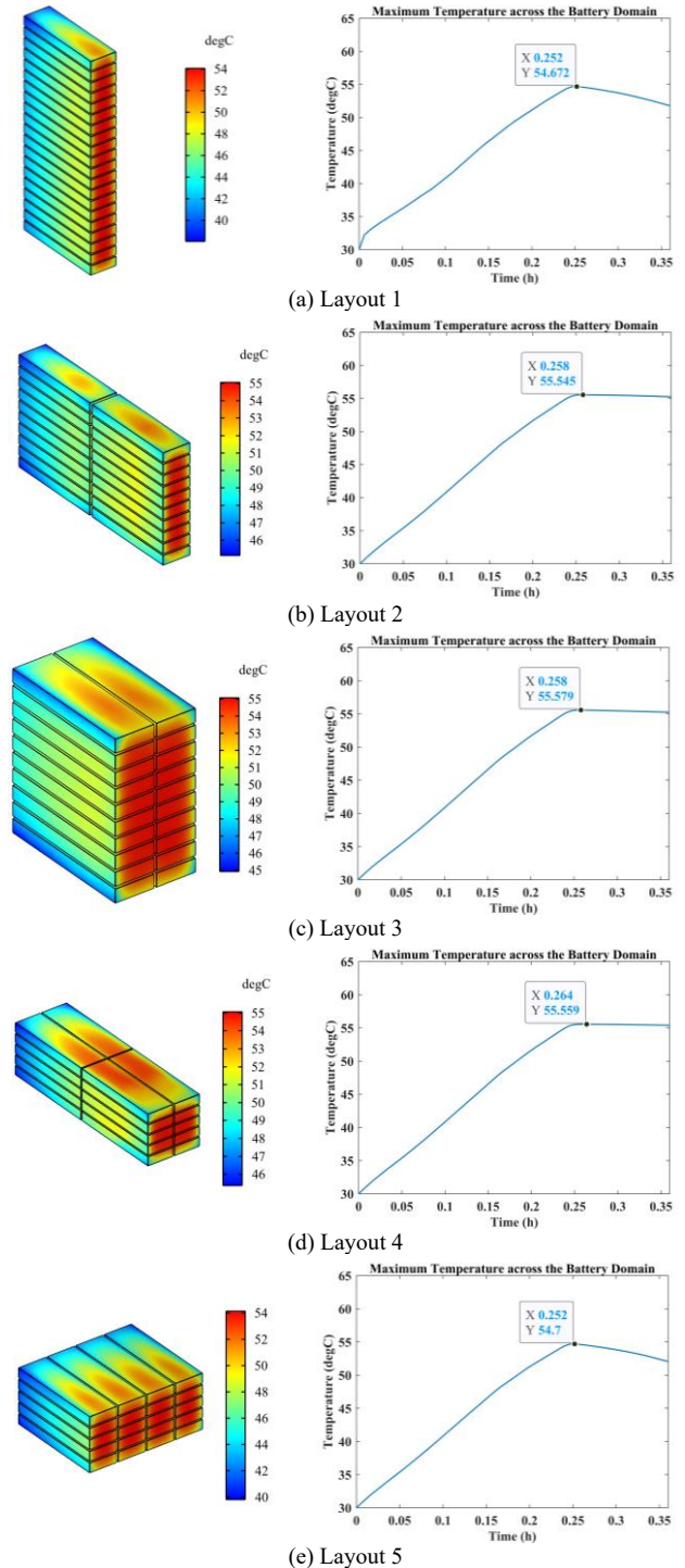
Fig. 5. The distribution of temperature across all battery packs with air cooling along the y-axis for 5 different layouts.
