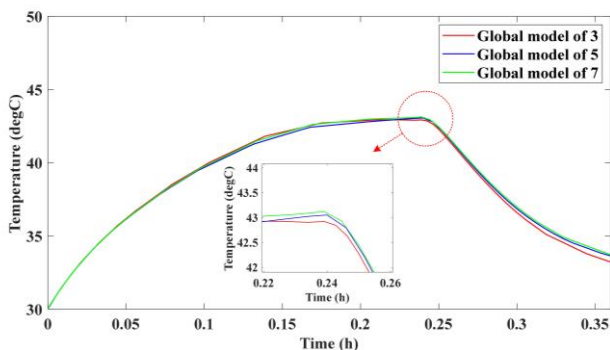
Fig. 7. The maximum temperature for full-scale models included in a global model of 3, 5 and 7 packs, respectively.
