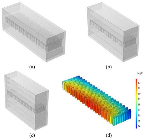
Fig. 6. (a) – (c) The full-scale model included in a global model of 3, 5 and 7. (d) The temperature distribution of the target pack in the full-scale model.
