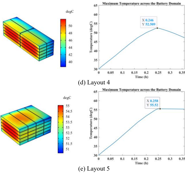
Fig. 4. The distribution of temperature across all battery packs with air cooling along the x-axis for 5 different layouts.
