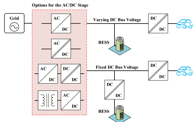
Fig. 1. Structures of EV fast chargers with the BESS.
