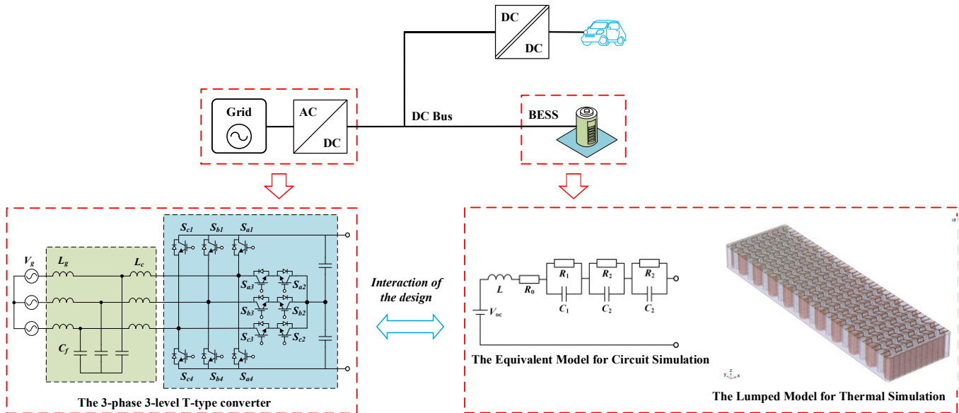
Fig. 3. The overall structure of the 450 kW EV fast chargers integrated with the BESS and the model used.
